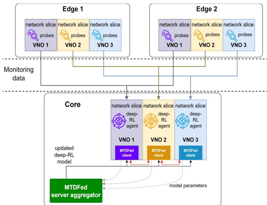
Figure 4: Architecture of the FL-based deep-RL training in NATWORK architecture.
